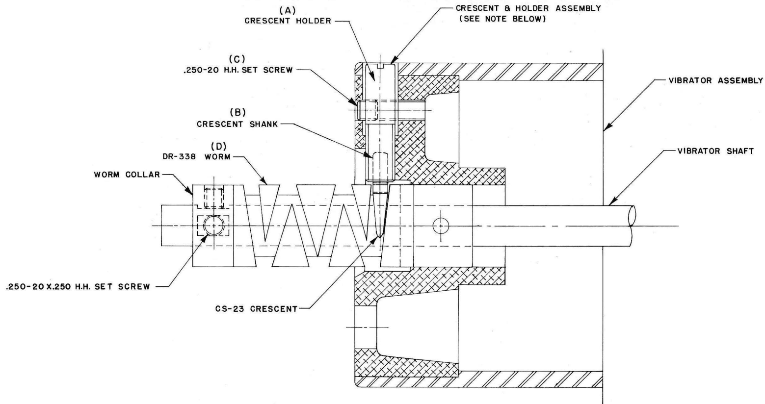
PARTIAL SECTION VIEW OF INK DRUM VIBRATOR ASSEMBLY
